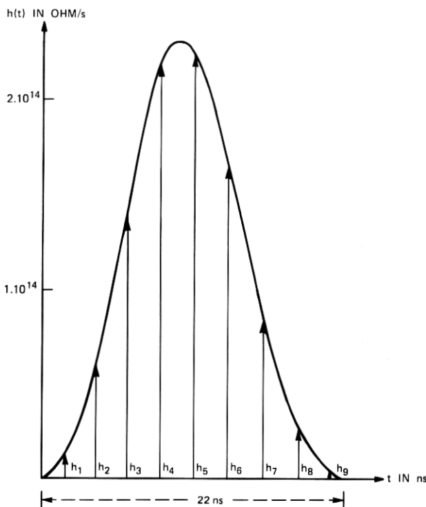
Fig. 10—Impulse response.
